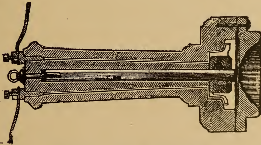
Fig. 29. BELL'S RECEIVER.
